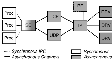
Figure 1: Design of the NewtOS network stack
